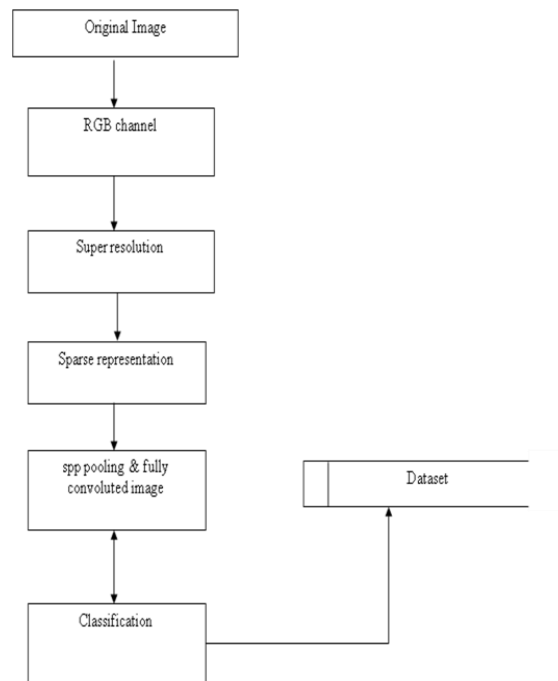
Figure 1: CNN
