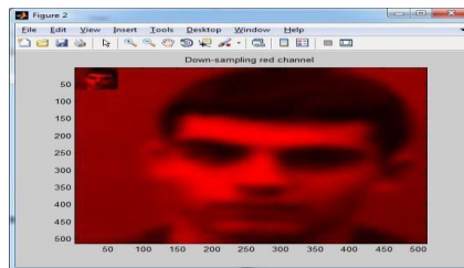
Figure 3: RGB Channel
