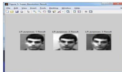
Figure 4: Super Resolution
